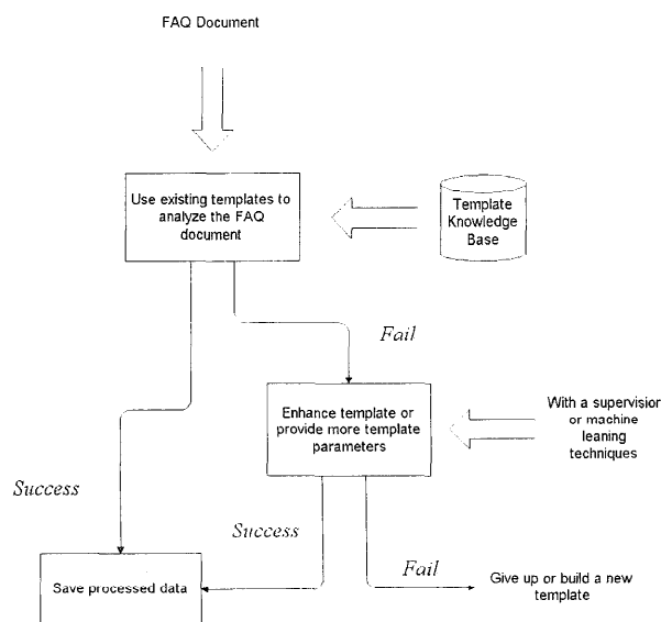
Figure 4: FAQ Miner Architecture
