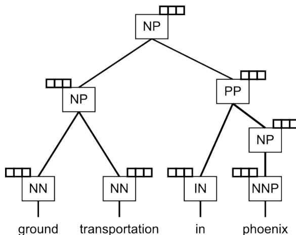
Fig. 1. Basic RecNN Structure
