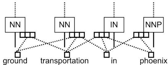
Fig. 4. Trigram Leaves
