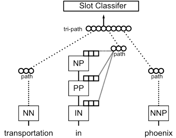
Fig. 3. Tri-path Features. The slot classifier is applied to each word in turn.
